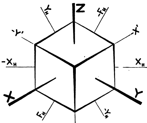
FIG. 10.—A rhombohedron projected along the trigonal axis on the (111) plane.
